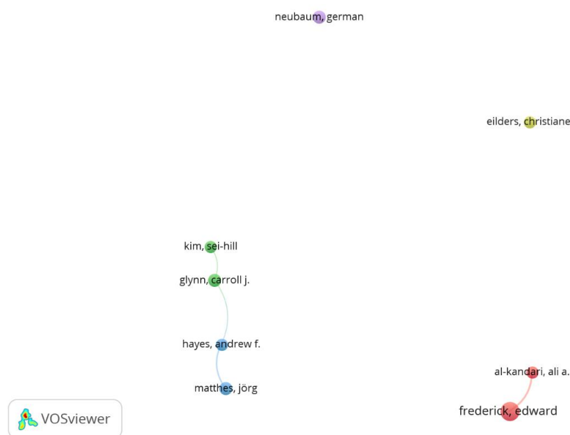
Figure 1. Author Visualization
