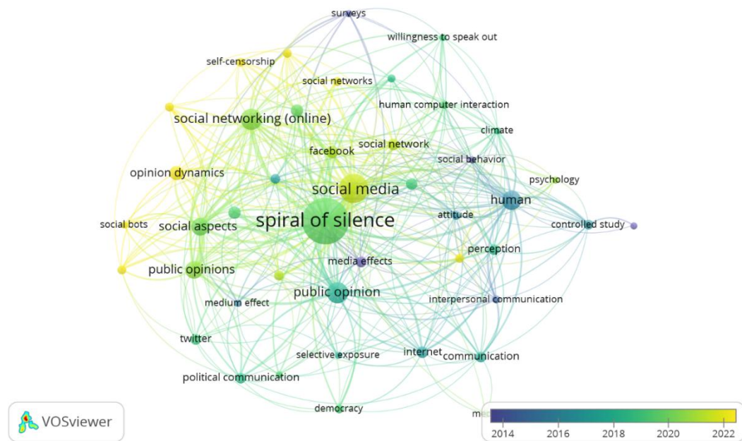
Figure 4. Overlay Visualization
