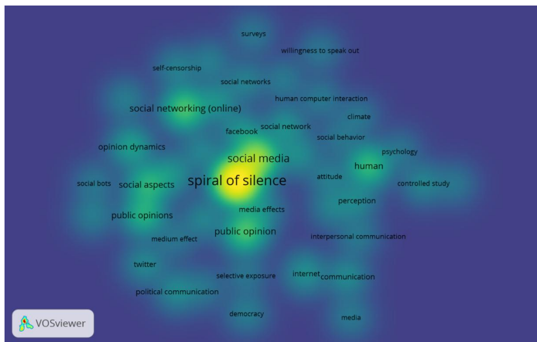
Figure 5. Density Visualization
